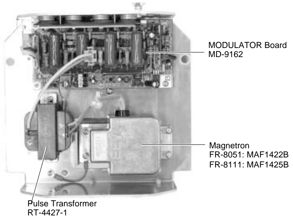
Figure 5-5 RF transceiver unit (FR-8051/8111), bottom view, cover removed
